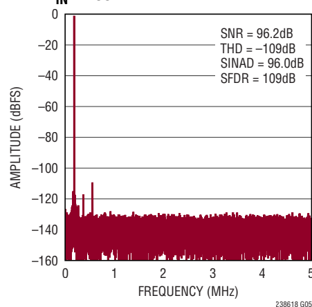
32k Point FFT f_{\text{SMPL}} = 10\text{Mps} , f_{\text{IN}} = 200\text{kHz}
