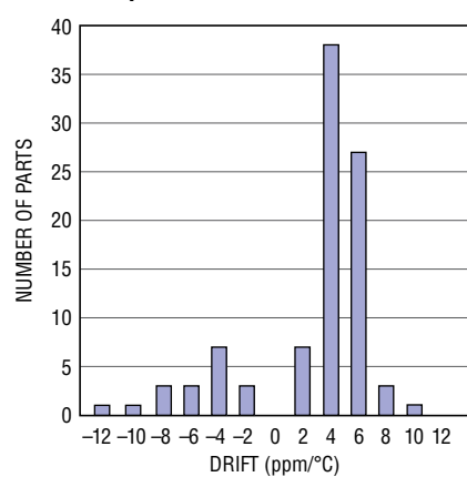
Internal Reference Output Temperature Coefficient Distribution
