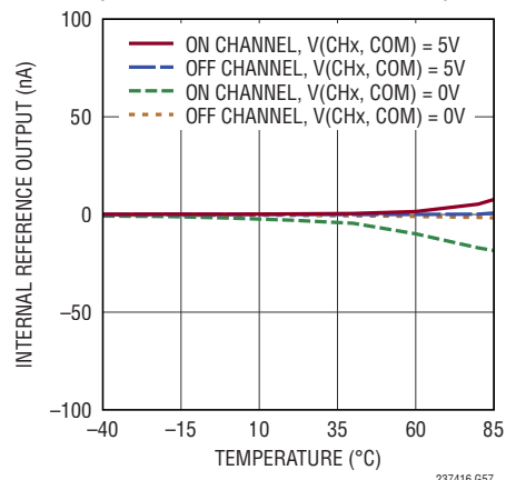
Input Leakage Current vs Temperature (MUXOUT± Shorted to ADCIN±)
