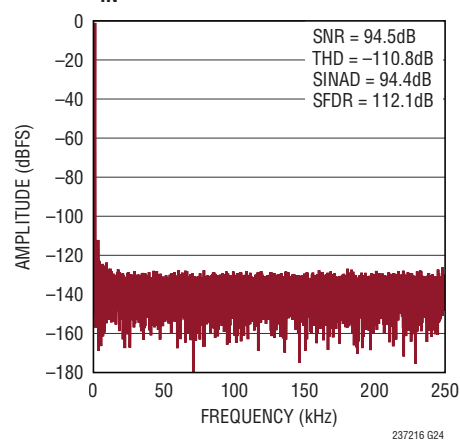
32k Point FFT f_{SAMPL} = 500\text{kps} , f_{IN} = 1\text{kHz} , REFBUF = 5\text{V}
