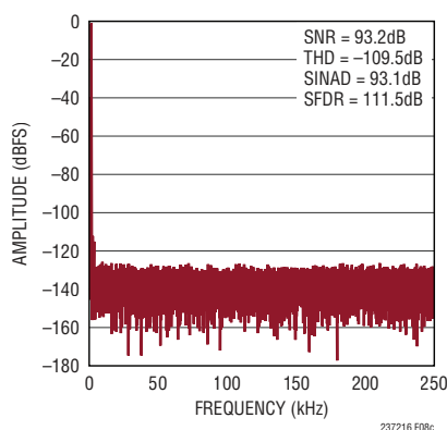
Figure 8c. 32k Point FFT f_{\text{SMP}} = 500\text{ksps} , f_{\text{IN}} = 1\text{kHz} for Circuit Shown in Figure 8a; Driven with Unipolar Inputs
