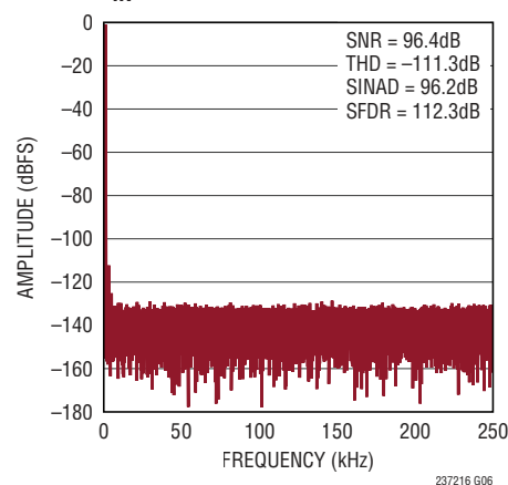
32k Point FFT f_{SAMPL} = 500\text{ksps} , f_{IN} = 1\text{kHz} , REF_{BUF} = 5\text{V}
