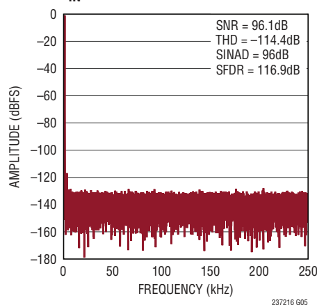
32k Point FFT f_{SAMPL} = 500\text{ksps} , f_{IN} = 1\text{kHz}
