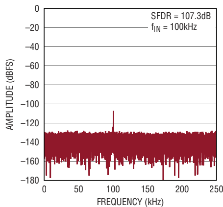
Crosstalk FFT (AC Crosstalk-Channel Adjacent to MUXOUT)
