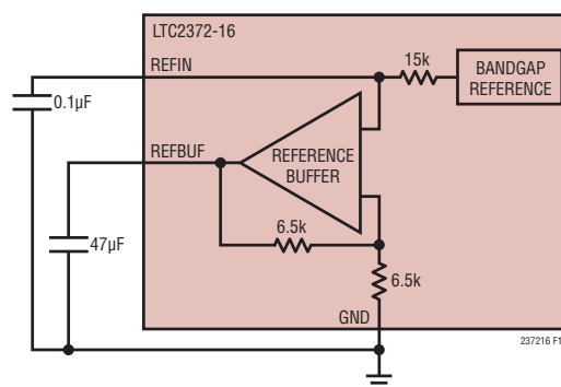
Figure 12a. LTC2372-16 Internal Reference Circuit
