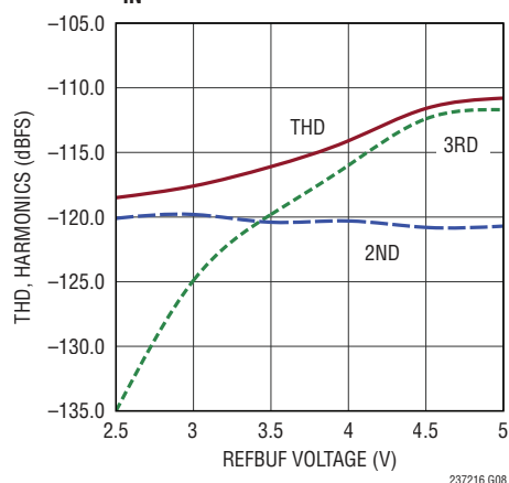
THD, Harmonics vs REF_{BUF} , f_{IN} = 1\text{kHz}
