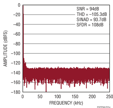
Figure 11c. 32k Point FFT f_{\text{SMPL}} = 500\text{ksps} , f_{\text{IN}} = 1\text{kHz} for Circuit Shown in Figure 11b
