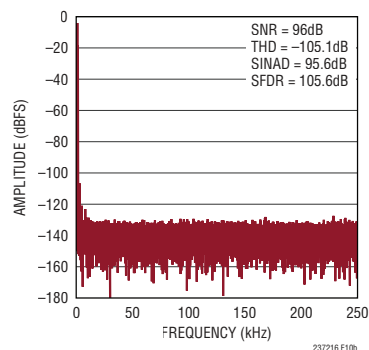
Figure 10b. 32k Point FFT f_{\text{SAMPL}} = 500\text{ksps} , f_{\text{IN}} = 1\text{kHz} for Circuit Shown in Figure 10a
