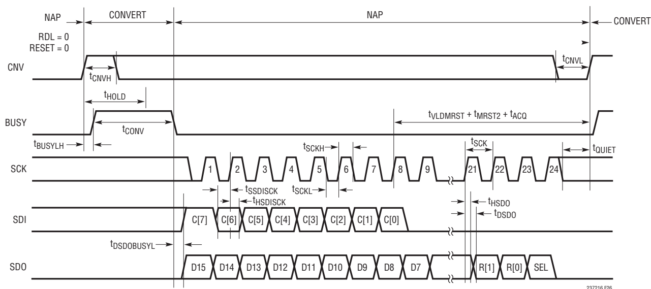
Figure 26. Using a Single LTC2372-16 Programming the Sequencer
