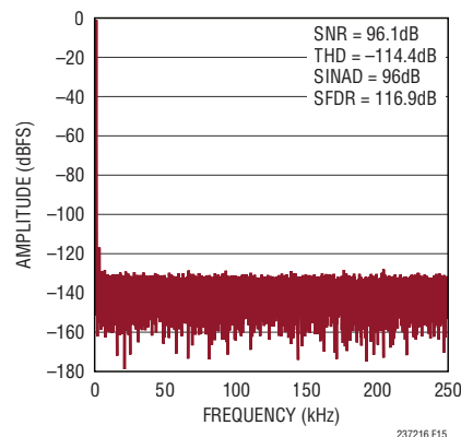
Figure 15. 32k Point FFT f_{SMP} = 500ksps , f_{IN} = 1kHz
