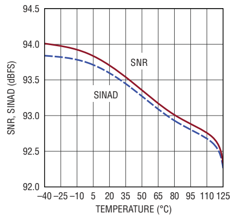
SNR, SINAD vs Temperature, f_{\text{IN}} = 1\text{kHz}
