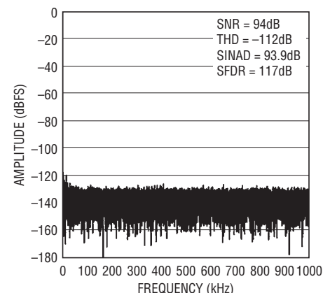
32k Point FFT f_{\text{S}} = 2\text{Msps} , f_{\text{IN}} = 2\text{kHz}
