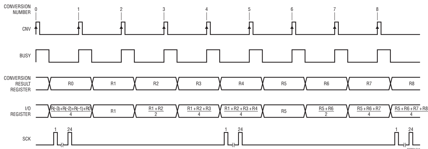
Figure 14. Averaging 4 Conversion Results
