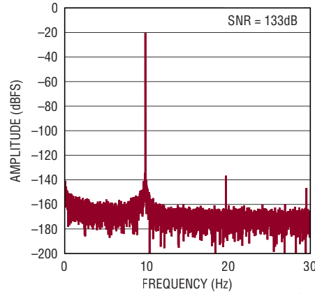
32k Point FFT f_{SAMPL} = 1\text{Mps} , f_{IN} = 10\text{Hz} , N = 16384
