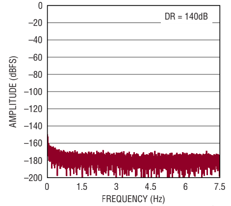
8k Point FFT f_{SAMPL} = 1\text{Mps} , IN^+ = \text{Near GND} , IN^- = \text{GND} , N = 65536
