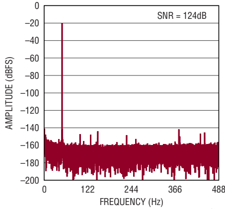
32k Point FFT f_{SAMPL} = 1\text{Mps} , f_{IN} = 50\text{Hz} , N = 1024
