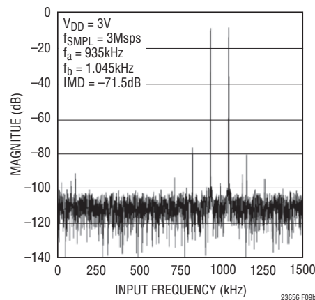
Figure 9b. LTC2366 Intermodulation Distortion Plot
