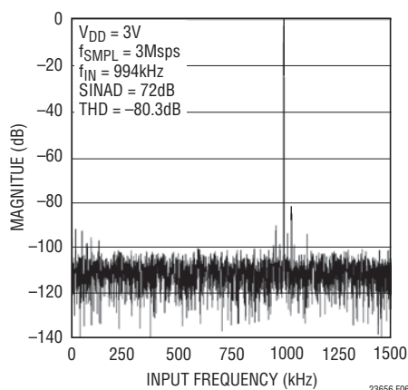
Figure 6. LTC2366 FFT Plot
