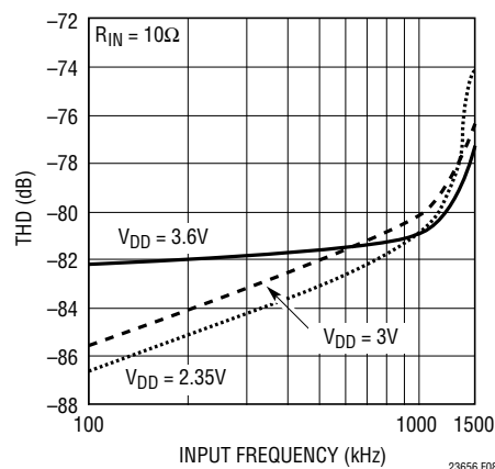
Figure 8. LTC2366 Distortion vs Input Frequency
