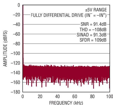
Figure 7c. \text{IN}^+/\text{IN}^- = 450\text{mV} 200Hz Fully Differential Sine, 0\text{V} \leq V_{\text{CM}} \leq 24\text{V} , 32k Point FFT, f_{\text{SAMPL}} = 200\text{ksps} . Circuit Shown in Figure 7a
