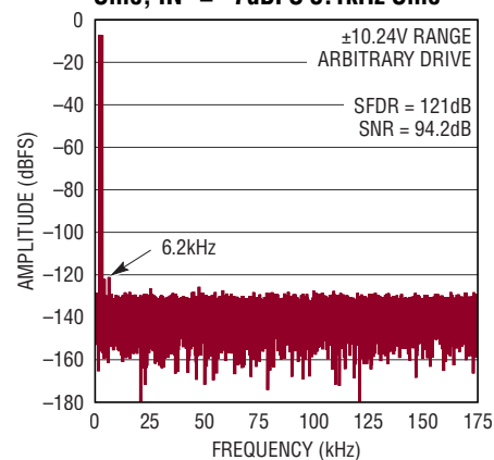
32k Point Arbitrary Two-Tone FFT f_{SAMPL} = 350\text{ksps} , IN^+ = -7\text{dBFS} 2kHz Sine, IN^- = -7\text{dBFS} 3.1kHz Sine
