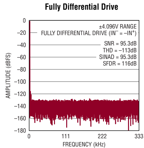
Figure 6c. IN^+/IN^- = -1dBFS 2kHz Fully Differential Sine, Common Mode = 2.5V, 32k Point FFT, f_{SAMPL} = 666ksps . Circuit Shown in Figure 6a with LT6237 Amplifiers, R_{FILT} = 24.9\Omega , C_{FILT} = 1nF
