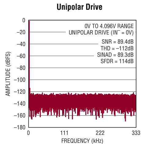
Figure 6e. IN^+ = -1dBFS 2kHz Unipolar Sine, IN^- = 0V , 32k Point FFT, f_{SAMPL} = 666ksps . Circuit Shown in Figure 6a with LT6237 Amplifiers, R_{FILT} = 24.9\Omega , C_{FILT} = 1nF
