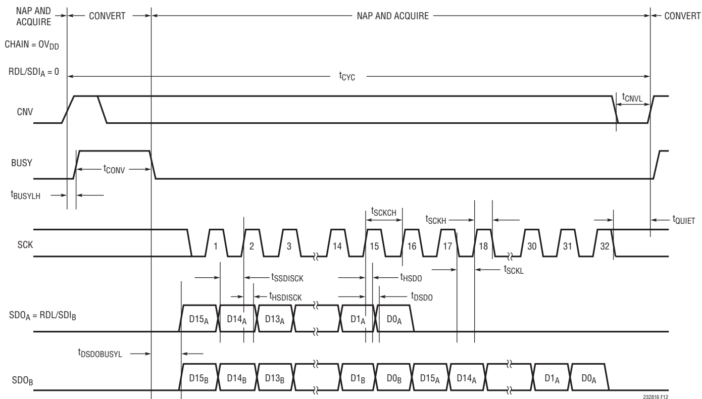
Figure 12. Chain Mode Timing Diagram
