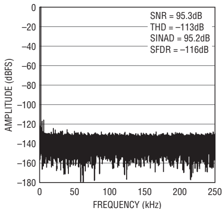
32k Point FFT f_S = 500\text{ksps} , f_{IN} = 2\text{kHz}
