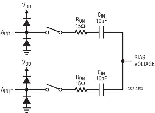
Figure 3. The Equivalent Circuit for the Differential Analog Input of the LTC2323-12
