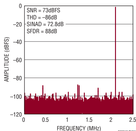
16k Point FFT f_s = 5\text{Mps} , f_{\text{IN}} = 2.2\text{MHz}
