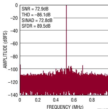
32k Point FFT f_s = 2\text{Mps} , f_{IN} = 500\text{kHz}
