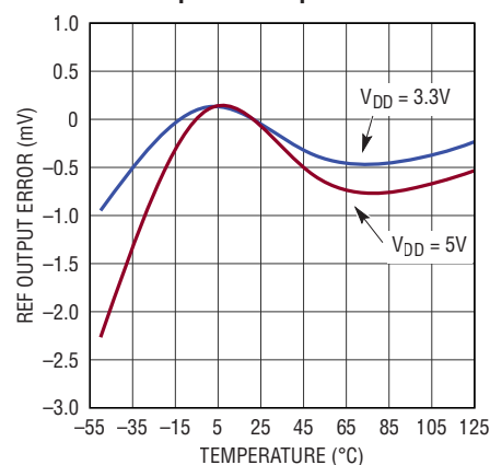
REF Output vs Temperature
