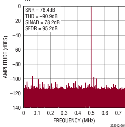
32k Point FFT, f_{\text{SMPL}} = 1.5\text{Mps} , f_{\text{IN}} = 500\text{kHz}
