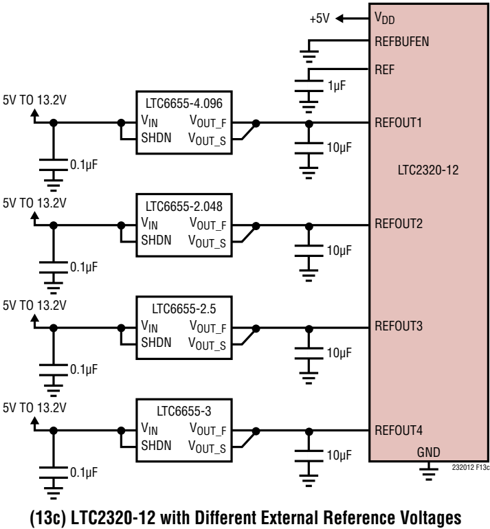
Figure 13. Reference Connections
