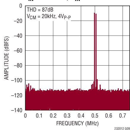
32k Point FFT, IMD, f_{\text{SMPL}} = 1.5\text{Mps} , A_{\text{IN}}^+ = 490\text{kHz} , A_{\text{IN}}^- = 510\text{kHz}
