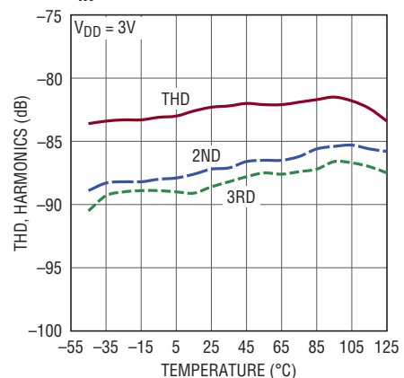
THD, Harmonics vs Temperature, f_{IN} = 500\text{kHz}
