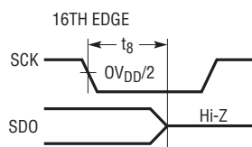
Figure 1. SDO Into Hi-Z after 16TH SCK↓
