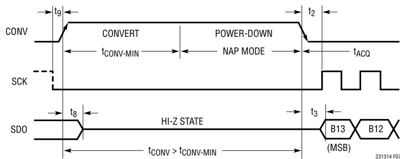
Figure 7. LTC2313-14 Nap Mode Power-Down Following Conversion for t_{\text{CONV}} > t_{\text{CONV-MIN}}
