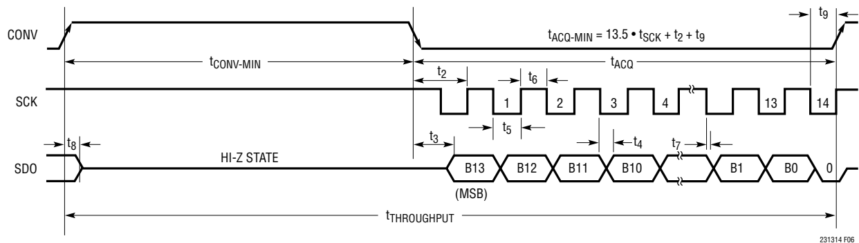
Figure 6. LTC2313-14 Serial Interface Timing Diagram (SCK High During t_{\text{CONV}} )
