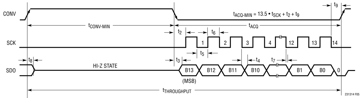
Figure 5. LTC2313-14 Serial Interface Timing Diagram (SCK Low During t_{\text{CONV}} )
