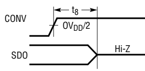
Figure 2. SDO Into Hi-Z After CONV↑
