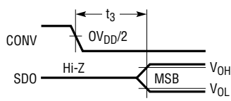
Figure 1. SDO Enabled After CONV↓
