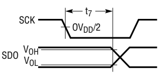
Figure 3. SDO Data Valid Hold After SCK↓
