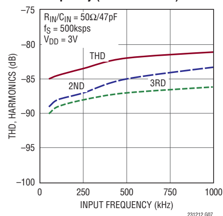
THD, Harmonics vs Input Frequency (50kHz to 1MHz)
