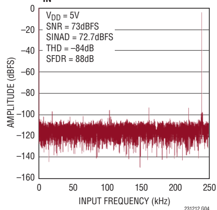
16k Point FFT, f_S = 500\text{kpsps} f_{IN} = 259\text{kHz}
