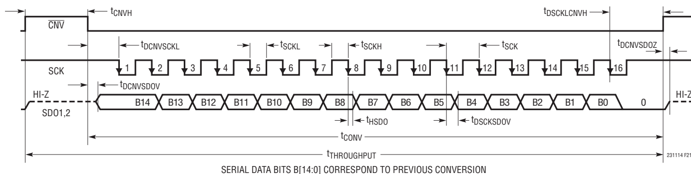
Figure 21. LTC2311-14 Timing Diagram, CMOS, LVDS I/O Modes
