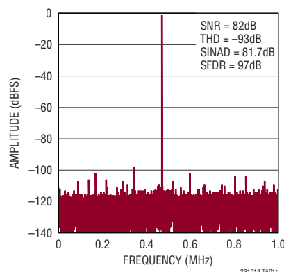
32k Point FFT f_{\text{SMP}} = 2\text{MSPs} , f_{\text{IN}} = 500\text{kHz}
