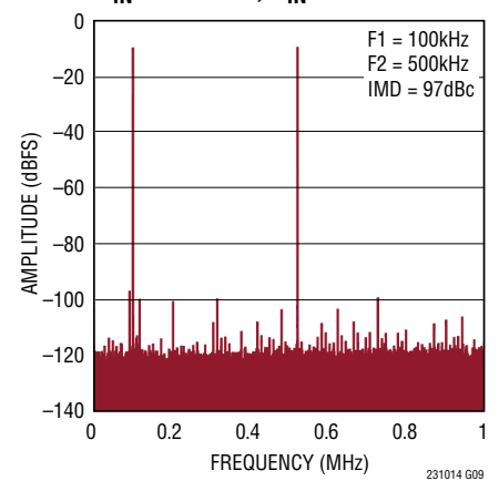
8k Point FFT, IMD, f_{\text{SAMPL}} = 2\text{MSPS} , A_{\text{IN}}^+ = 100\text{kHz} , A_{\text{IN}}^- = 500\text{kHz}
