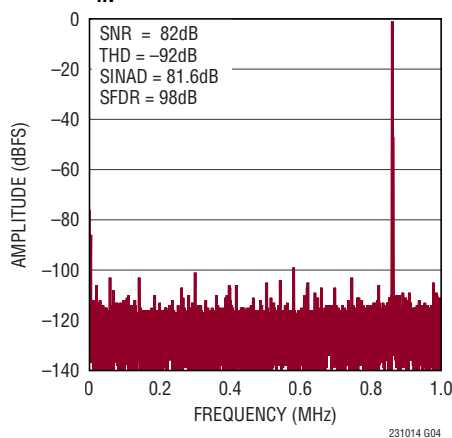
32k Point FFT, f_{\text{SAMPL}} = 2\text{MSPS} , f_{\text{IN}} = 1150\text{kHz}
