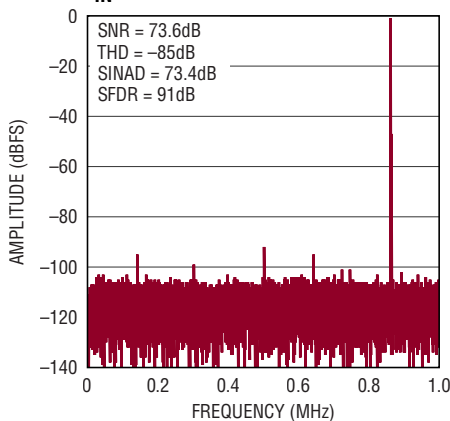
32k Point FFT, f_{\text{SAMPL}} = 2\text{MSPS} , f_{\text{IN}} = 1150\text{kHz}
