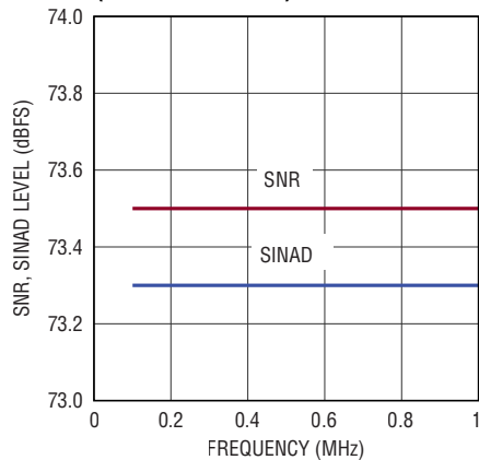
SNR, SINAD vs Input Frequency (100kHz to 1MHz)
