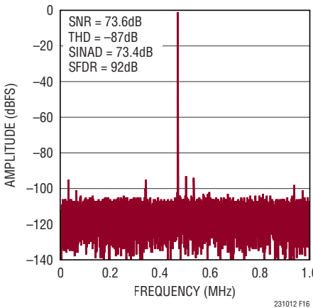
Figure 16. 32k Point FFT of the LTC2310-12
