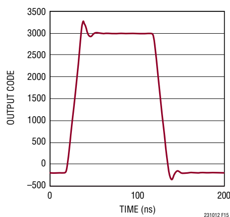
Figure 15. Transient Response of the LTC2310-12
