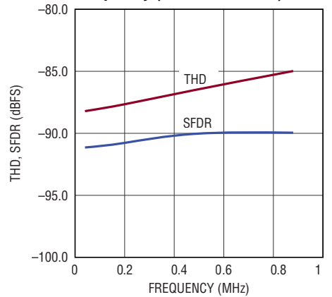
THD, Harmonics vs Input Frequency (100kHz to 1MHz)
