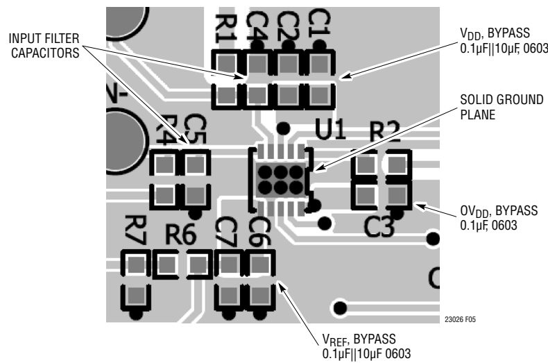
Figure 5. Suggested Layout
