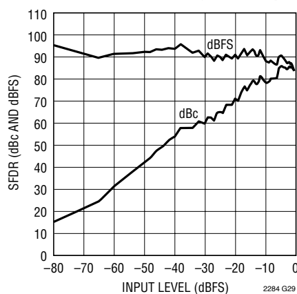
SFDR vs Input Level, f_{IN} = 70\text{MHz} , 2V Range, 105Mps
