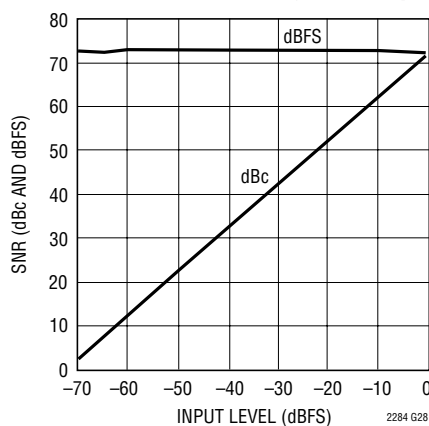
SNR vs Input Level, f_{IN} = 70\text{MHz} , 2V Range, 105Mps
