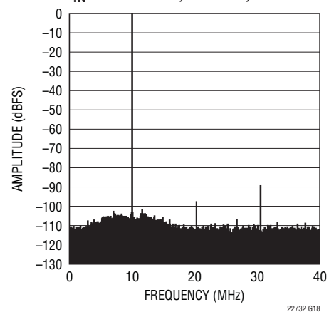
LTC2273: 64k Point FFT, f_{IN} = 170.2MHz , -1dBFS, PGA = 1
