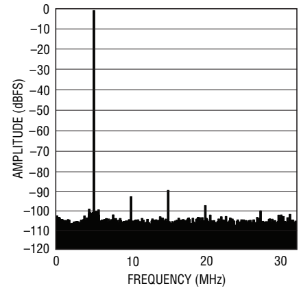
LTC2265-14: 8k Point FFT, f_{IN} = 5\text{MHz} , -1\text{dBFS} , 65Mps
