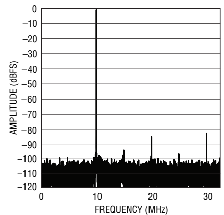
LTC2265-14: 8k Point FFT, f_{IN} = 140\text{MHz} , -1\text{dBFS} , 65Mps
