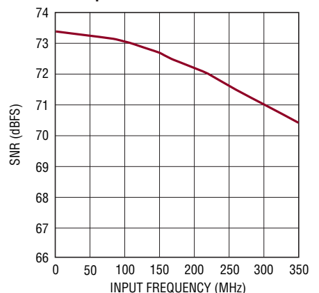
LTC2264-14: SNR vs Input Frequency, -1\text{dBFS} , 2\text{V} Range, 40\text{Mps}
