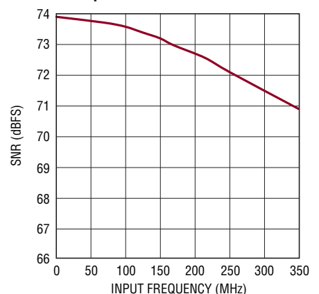
LTC2265-14: SNR vs Input Frequency, -1\text{dBFS} , 2V Range, 65Mps
