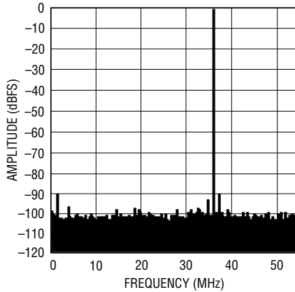
LTC2260-14: 8k Point FFT, f_{IN} = 70\text{MHz} -1dBFS, 105Msps
