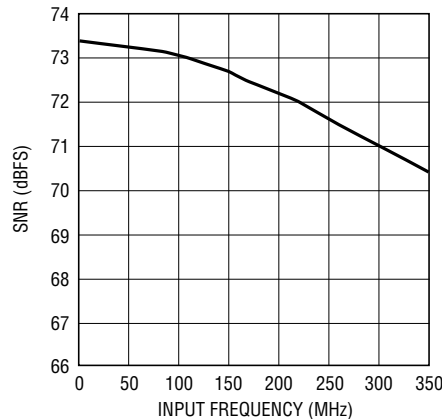
LTC2260-14: SNR vs Input Frequency, -1dB, 2V Range, 105Msps
