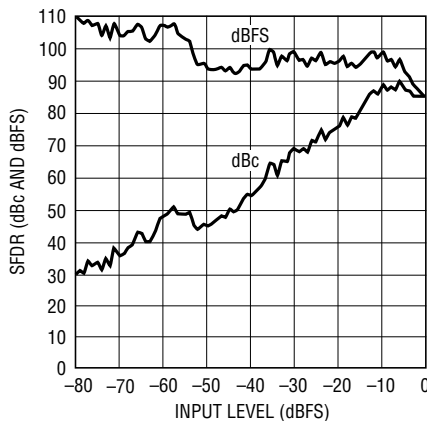
LTC2260-14: SFDR vs Input Level, f_{IN} = 70\text{MHz}, 2\text{V Range}, 105\text{Msps}
