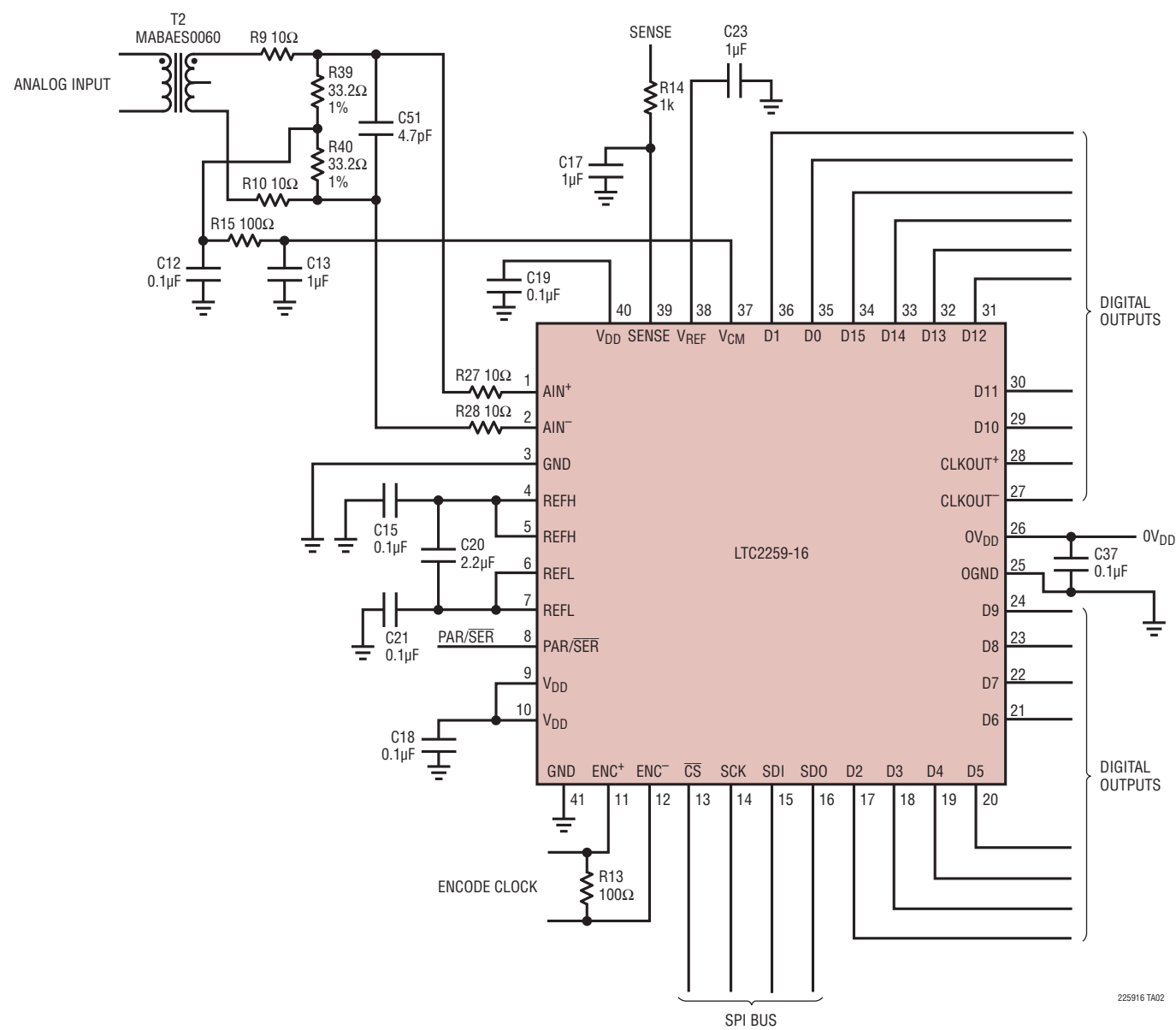
LTC2259-16 Schematic
