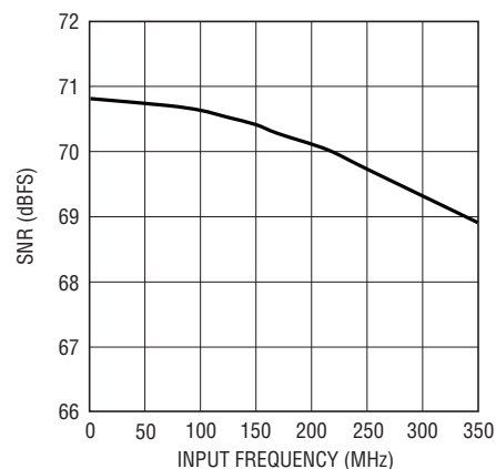
LTC2260-12: SNR vs Input Frequency, -1dB, 2V Range, 105\text{Mpsps}
