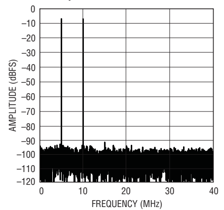
LTC2259-12: 8k Point 2-Tone FFT, f_{IN} = 70\text{MHz} , 75\text{MHz} , -1\text{dBFS} , 80\text{Mpsps}
