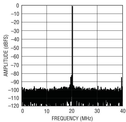
LTC2259-12: 8k Point FFT, f_{IN} = 140\text{MHz} , -1\text{dBFS} , 80\text{Mpsps}
