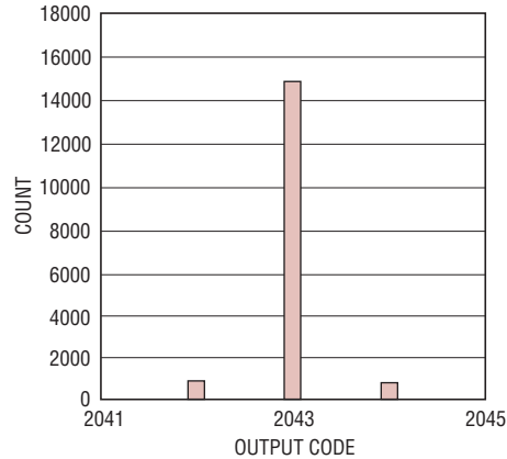
LTC2261-12: Shorted Input Histogram
