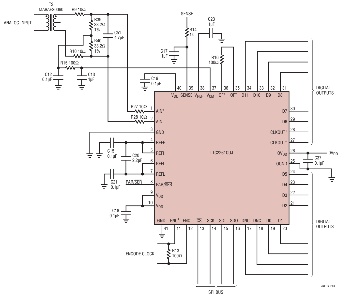
LTC2261 Schematic
