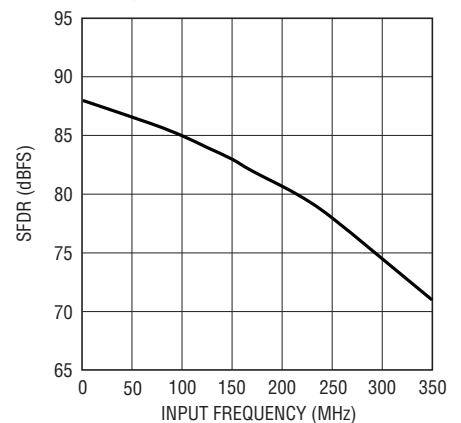
LTC2259-12: SFDR vs Input Frequency, -1\text{dB} , 2\text{V} Range, 80\text{Mpsps}
