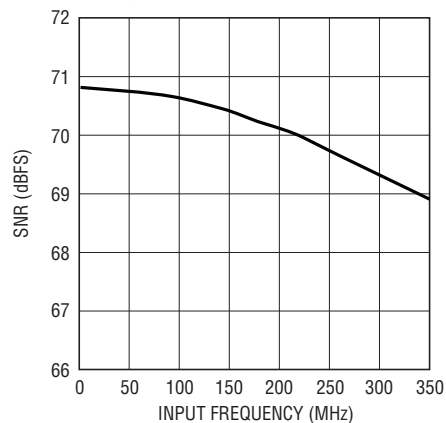
LTC2259-12: SNR vs Input Frequency, -1\text{dB} , 2\text{V} Range, 80\text{Mpsps}
