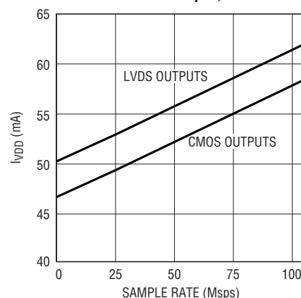
LTC2260-12: I_{VDD} vs Sample Rate, 5\text{MHz Sine Wave Input, -1dB}
