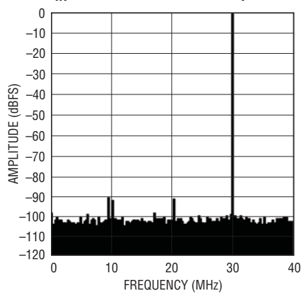
LTC2259-16: 8k Point FFT, f_{IN} = 30\text{MHz} -1dBFS, 80Mps
