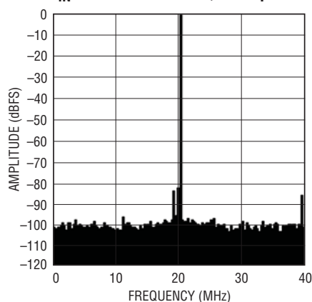
LTC2259-16: 8k Point FFT, f_{IN} = 140\text{MHz} -1dBFS, 80Mps
