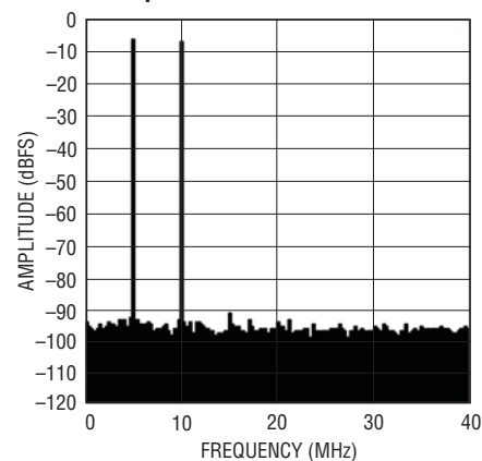
LTC2259-16: 8k Point 2-Tone FFT, f_{IN} = 70\text{MHz}, 75\text{MHz} , -1dBFS, 80Mps
