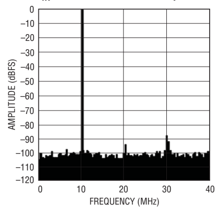
LTC2259-16: 8k Point FFT, f_{IN} = 70\text{MHz} -1dBFS, 80Mps
