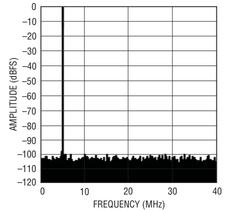
LTC2259-16: 8k Point FFT, f_{IN} = 5\text{MHz} -1dBFS, 80Mps
