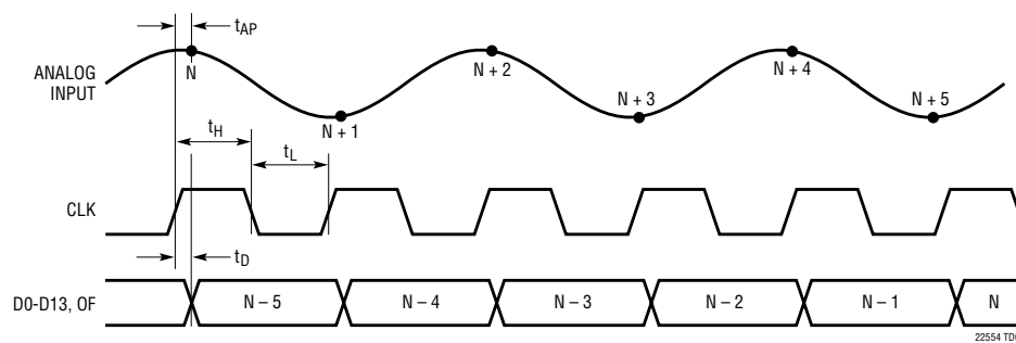
Timing Diagram
