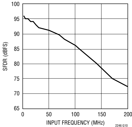
LTC2246: SFDR vs Input Frequency, -1dB, 2V Range, 25Mps
