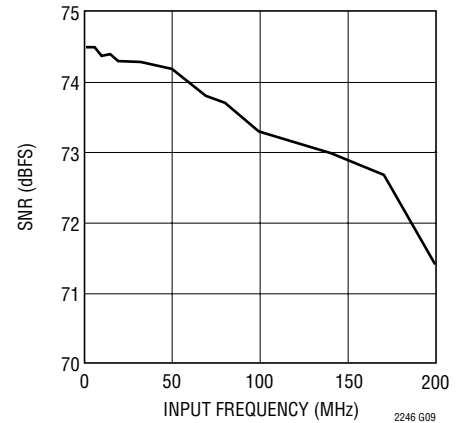
LTC2246: SNR vs Input Frequency, -1dB, 2V Range, 25Mps
