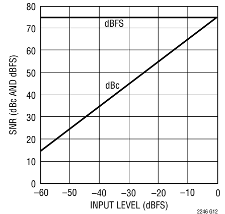
LTC2246: SNR vs Input Level, f_{IN} = 5\text{MHz} , 2V Range, 25Mps
