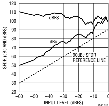
LTC2246: SFDR vs Input Level, f_{IN} = 5\text{MHz} , 2V Range, 25Mps
