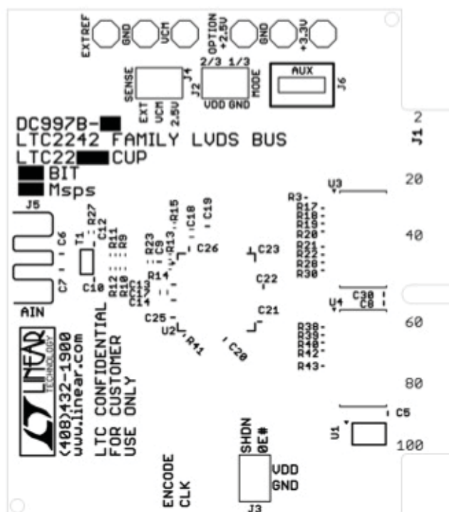
Silkscreen Top
