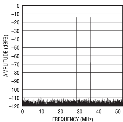
LTC2207-14: 32K Point 2-Tone FFT, f_{IN} = 69.2\text{MHz} and 76.5\text{MHz} , -15\text{dBFS} , \text{PGA} = 0 , RAND "On", Dither "Off"
