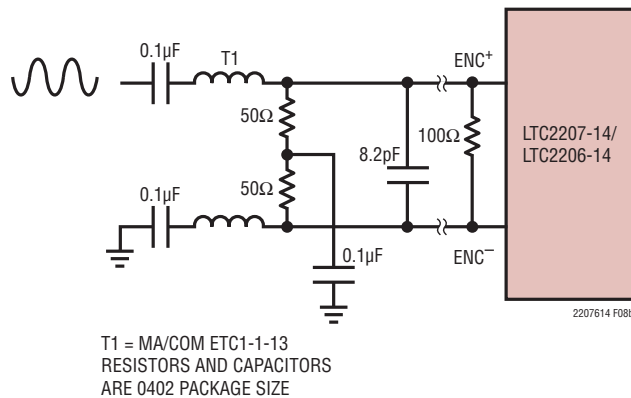
Figure 8b. Transformer Driven Encode
