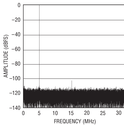
LTC2205: 64K Point FFT, 65Mps, f_{IN} = 5.1\text{MHz} , -1dBFS, PGA = 1, DITH = 0
