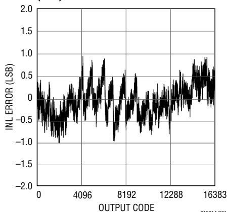
LTC2153-14: Integral Nonlinearity (INL)
