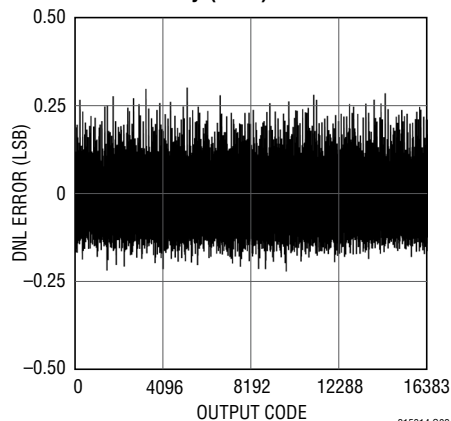
LTC2153-14: Differential Nonlinearity (DNL)
