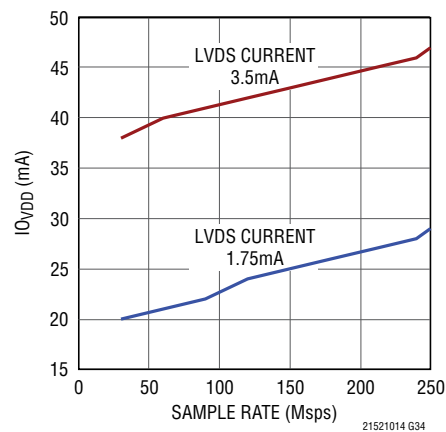
LTC2151-14: I_{QDD} vs Sample Rate, 15MHz Sine Wave Input, -1\text{dBFS}
