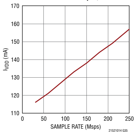
LTC2151-14: I_{QDD} vs Sample Rate, 15MHz Sine Wave Input, -1\text{dBFS}
