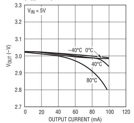
-3V OUT vs I_{OUT} Over Temperature ( V_{IN} = 5\text{V} )
