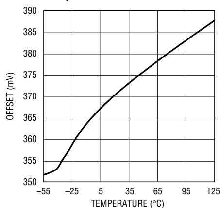
Ramp Offset Voltage vs Temperature
