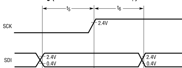
t 5 (SDI Setup Time Before SCK↑), t 6 (SDI Hold Time After SCK↑)
