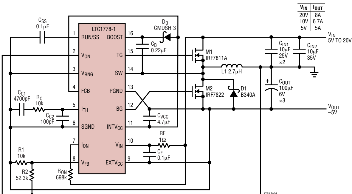
Positive-to-Negative Converter, -5\text{V}/5\text{A} at 300\text{kHz}
