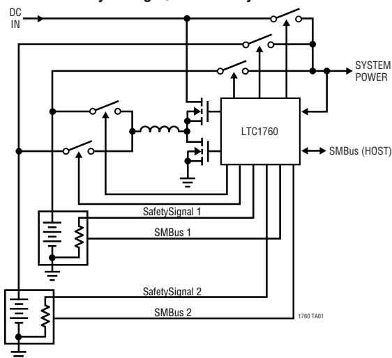
Dual Battery Charger/Selector System Architecture
