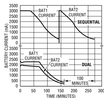
Dual vs Sequential Charging
