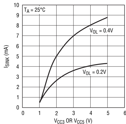
\overline{RST} , COMPX I_{SINK} vs Supply Voltage
