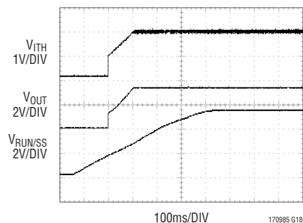
Soft-Start Up
