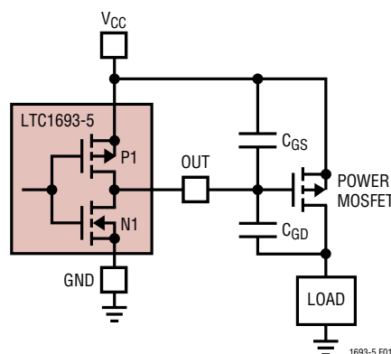
Figure 1. Capacitance Seen by OUT During Switching
