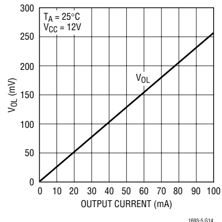
V_{OL} vs Output Current
