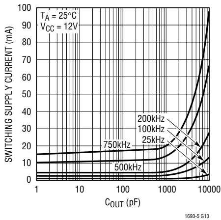
Switching Supply Current vs C_{OUT}
