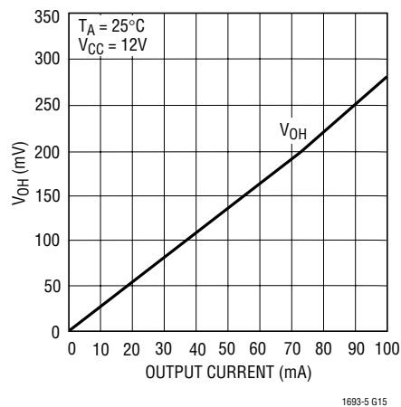
V_{OH} vs Output Current
