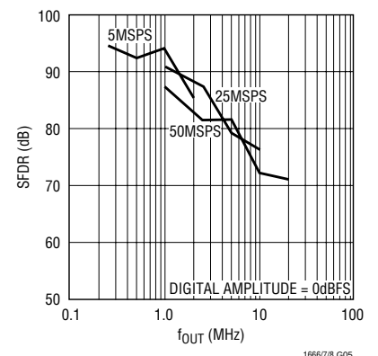
LTC1668 SFDR vs f_{OUT} and f_{CLOCK}
