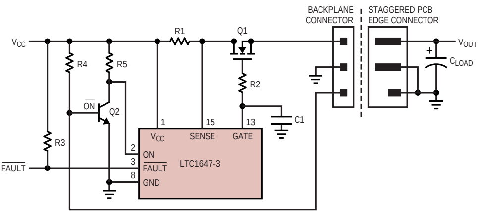
(a) HOT SWAP CONTROLLER ON MOTHERBOARD
