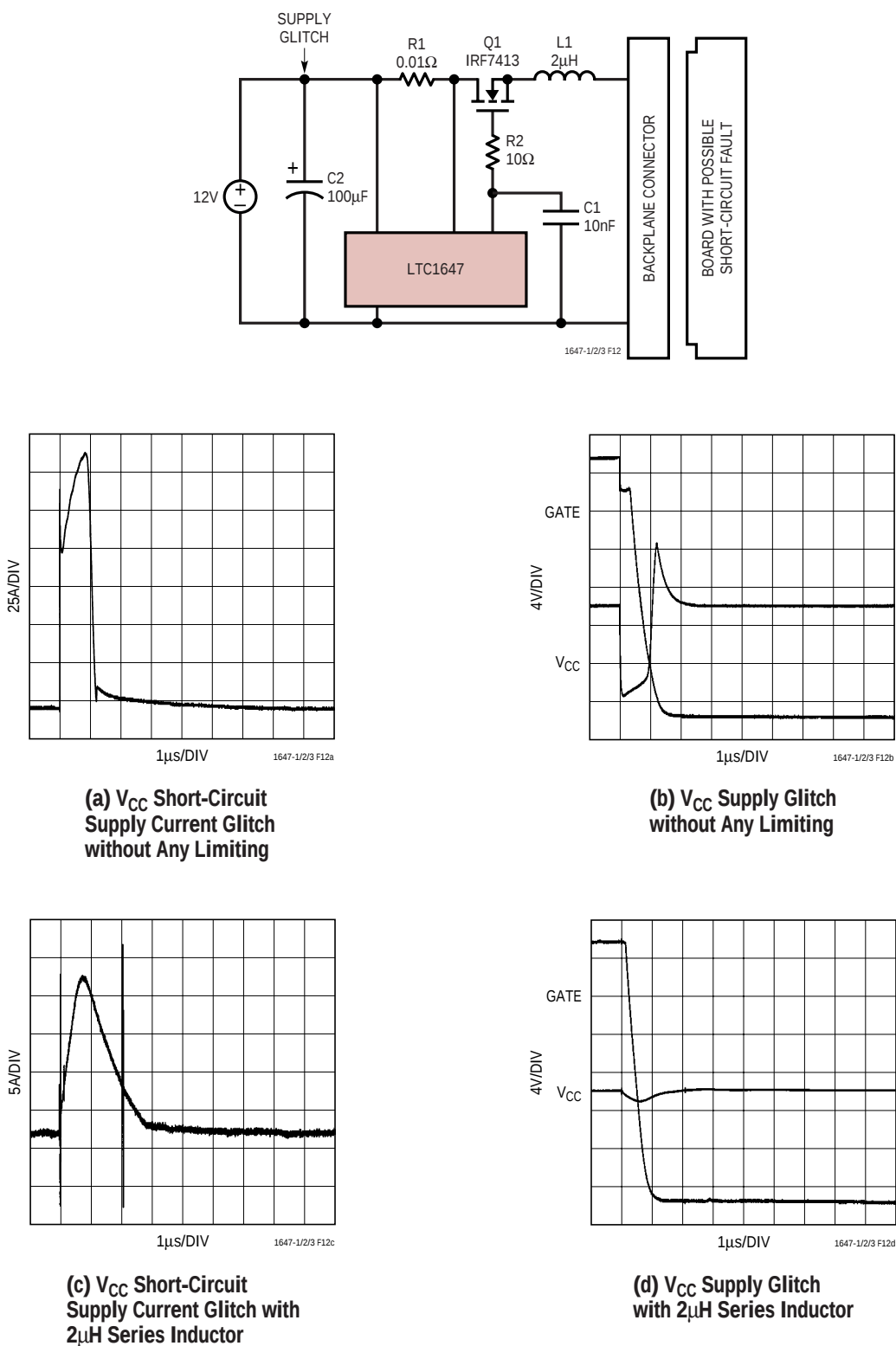
Figure 12. Supply Glitch
