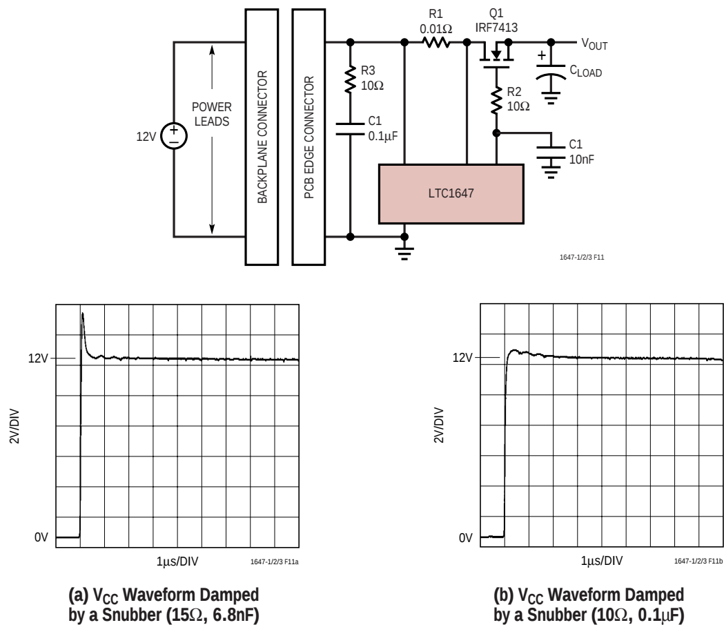
Figure 11. Snubber "Fixes"
